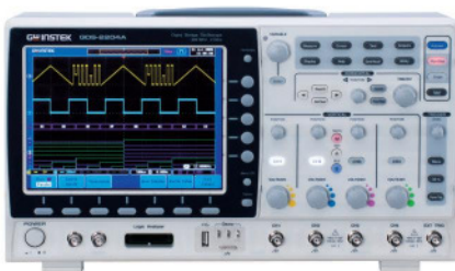
4 Channel Model
